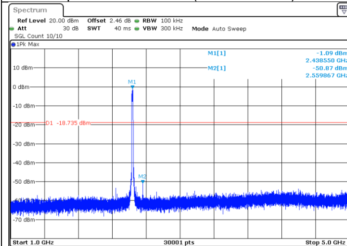
Spurious Emission (1GHz – 5GHz)
