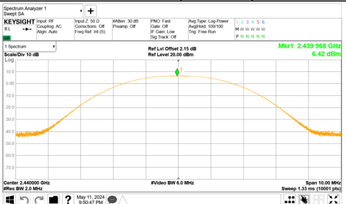
Channel 19 (2440MHz)
