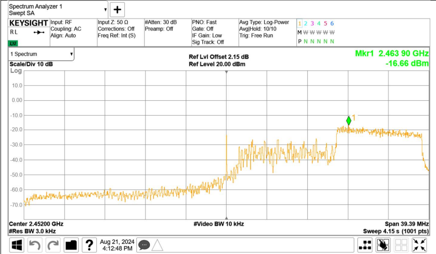
PSD NVNT ax40 2452MHz Ant1 RU106_56
