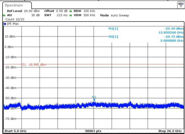
Spurious Emission (5GHz –26.5GHz)
