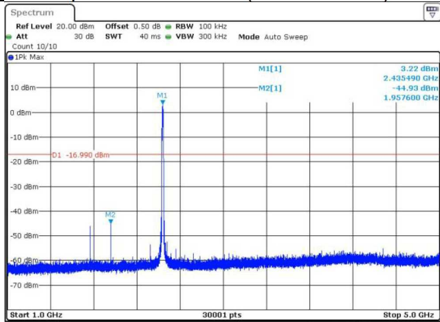
Spurious Emission (1GHz –5GHz)
