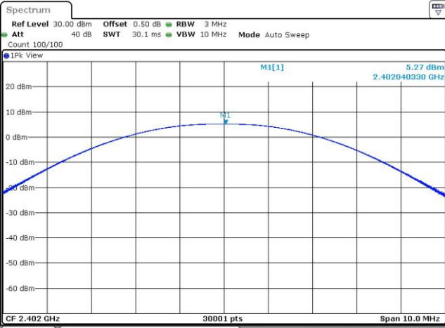
Channel 0 (2402MHz)
