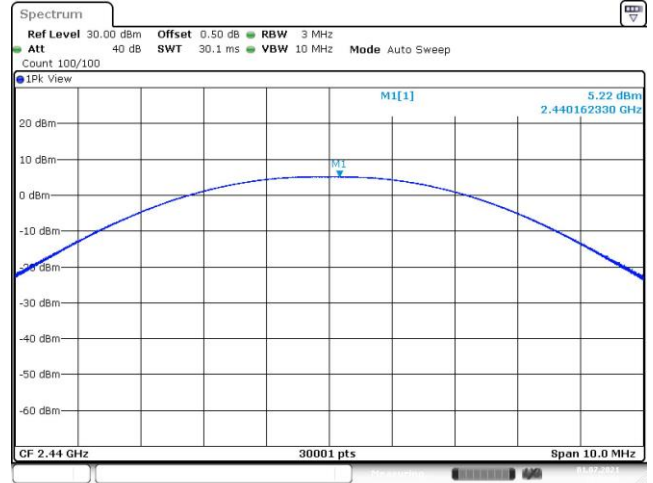
Channel 19 (2440MHz)
