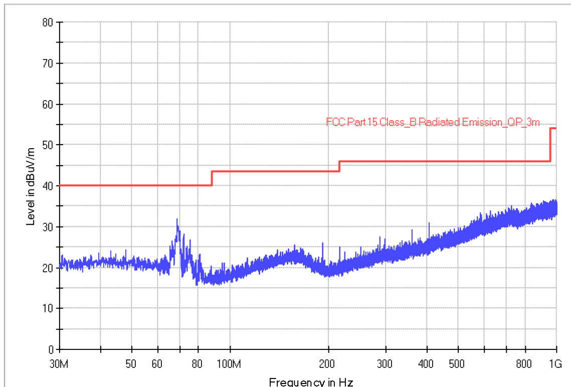
RE_VULB9168_pre_Conrt_30-1000
