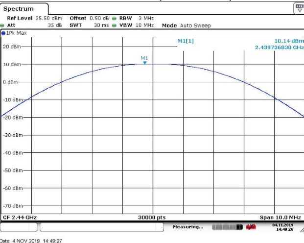
Channel 19 (2440MHz)
