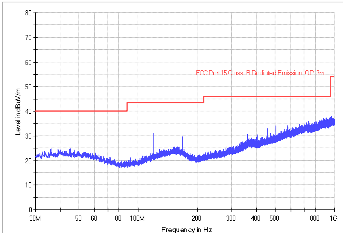
RE_VULB9168_pre_Cbnt_30-1000
