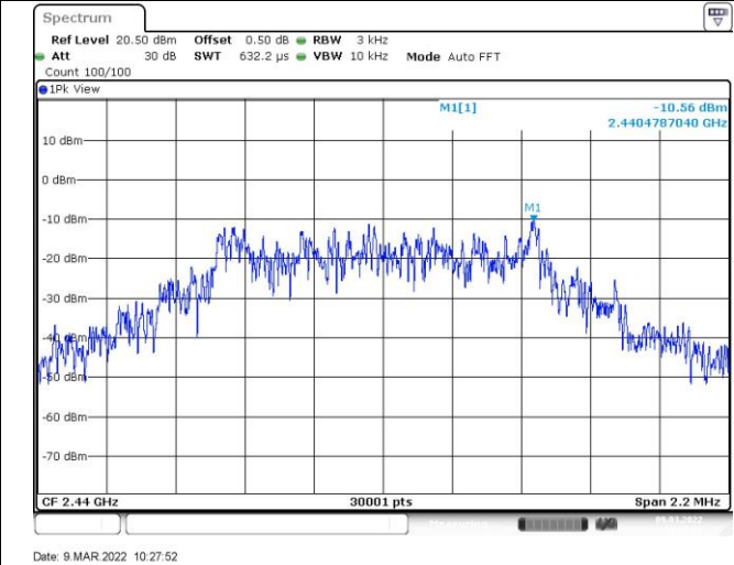
Channel 19 (2440MHz)
