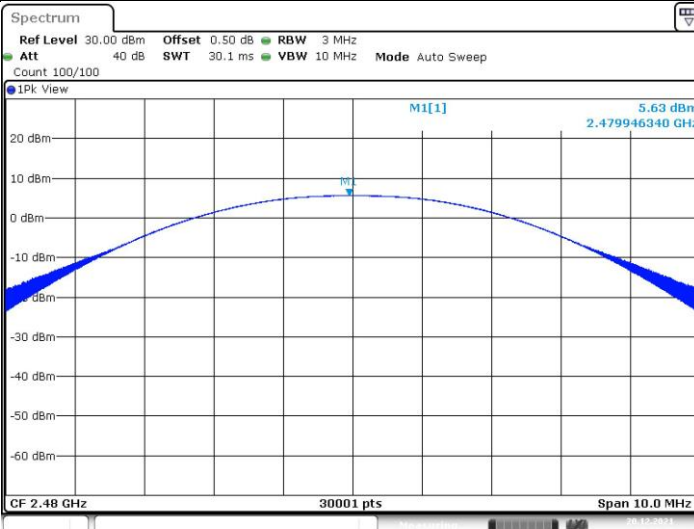
Channel 39 (2480MHz)
