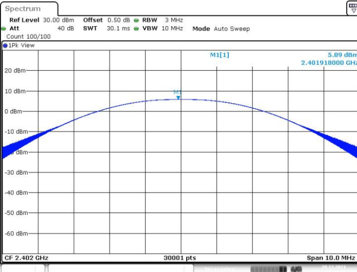
Channel 0 (2402MHz)
