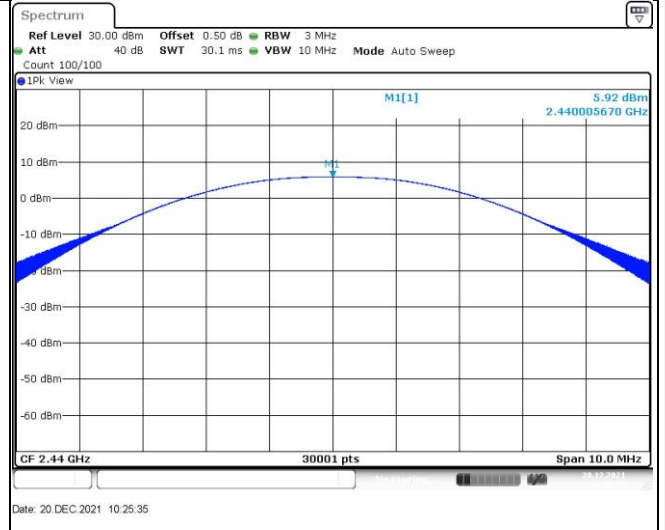
Channel 19 (2440MHz)
