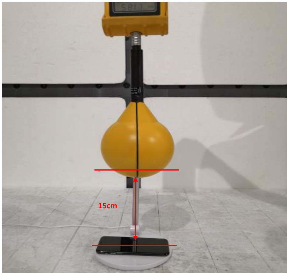
TestPosition E-Exposure photo from top surface (15cm) (TM1)
