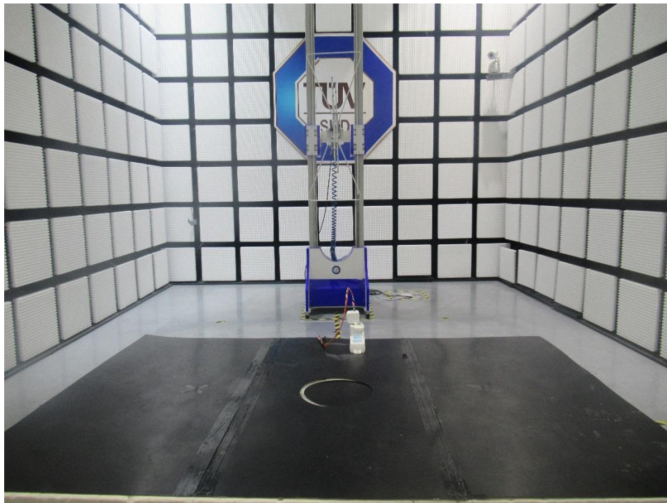
Radiated emissions 30MHz to 1000MHz
