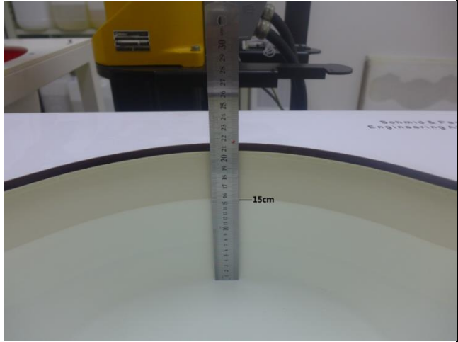
Photo 14: Tissue Simulant Liquid for Body 5G
