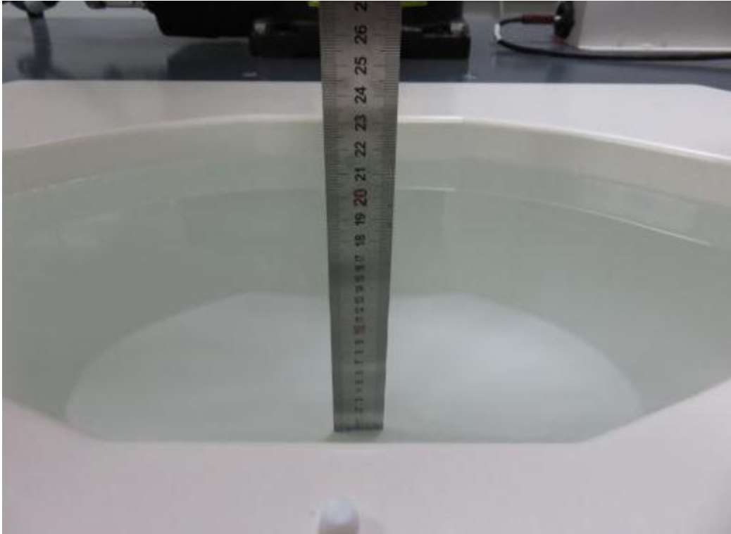
Photograph of the depth in the Body Phantom (450MHz-10000MHz, 16.2cm depth)
