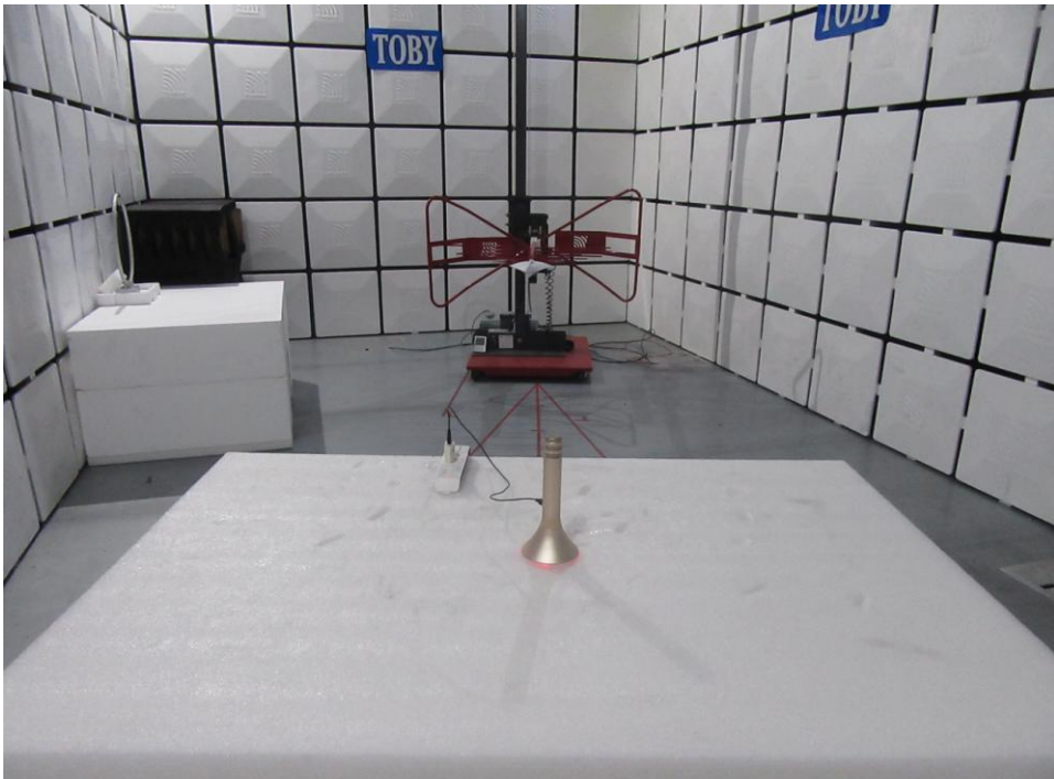
Test Setup
