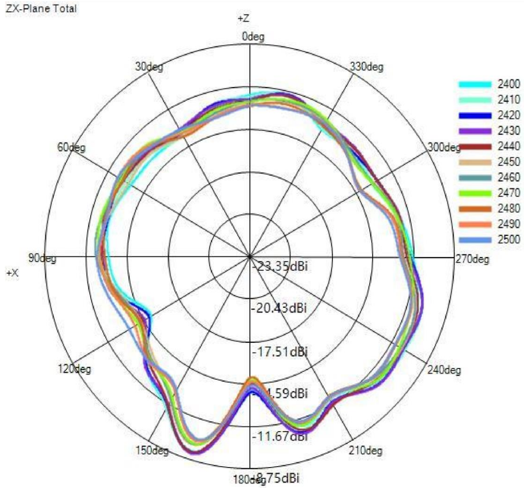
(1) X-Z Plane(unit:dBi):
