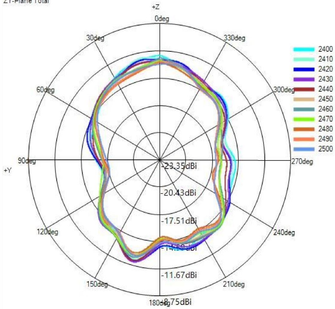
(2) Y-Z Plane(unit:dBi):
