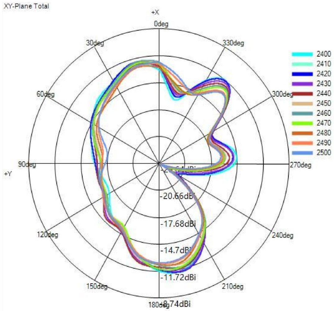
(3) X-Y Plane(unit:dBi):
