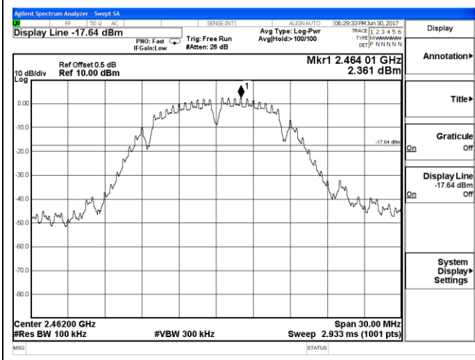
802.11b_High Channel
