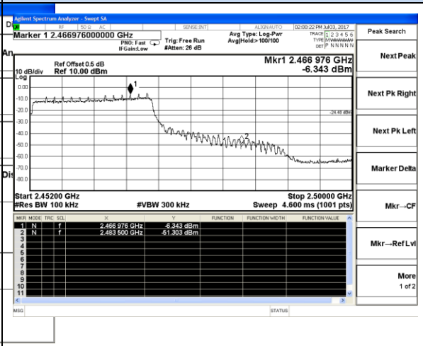
802.11n(HT40)-High channel
