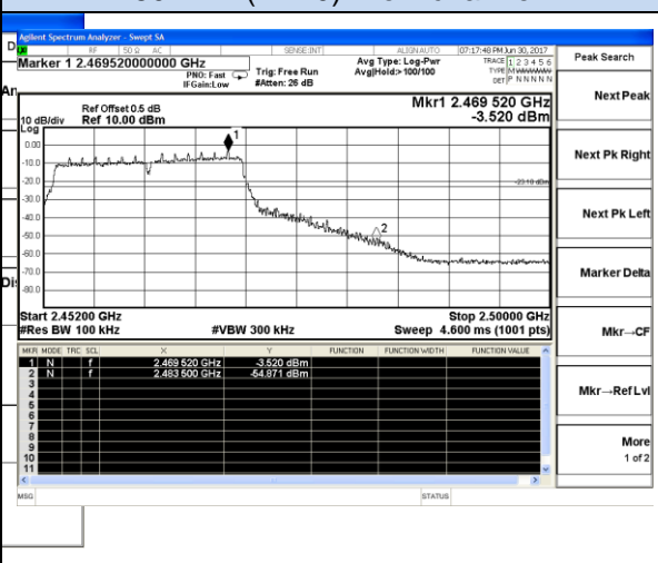
802.11n(HT20)-High channel
