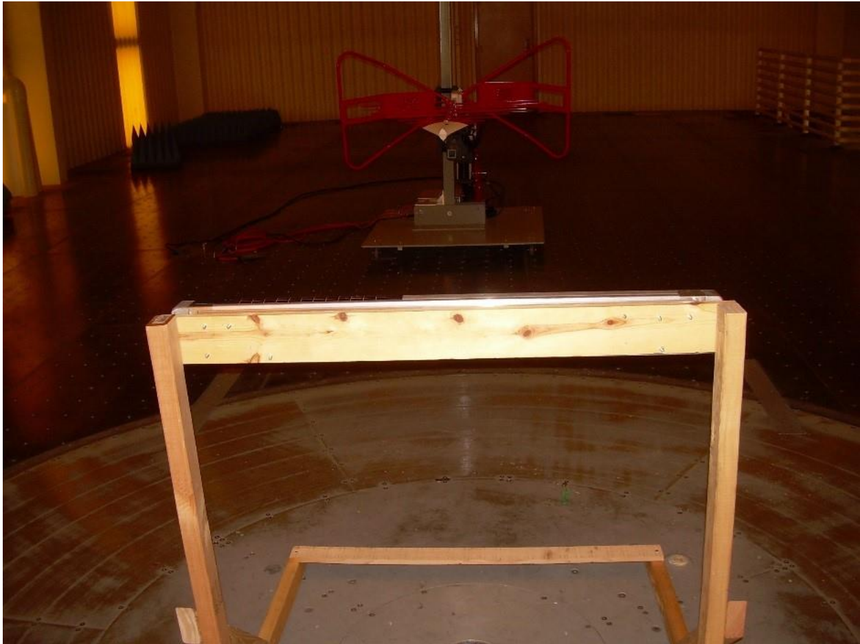
Photograph 2. Back View Radiated Emissions 30 to 1000 MHz Range – Awning Retracted
