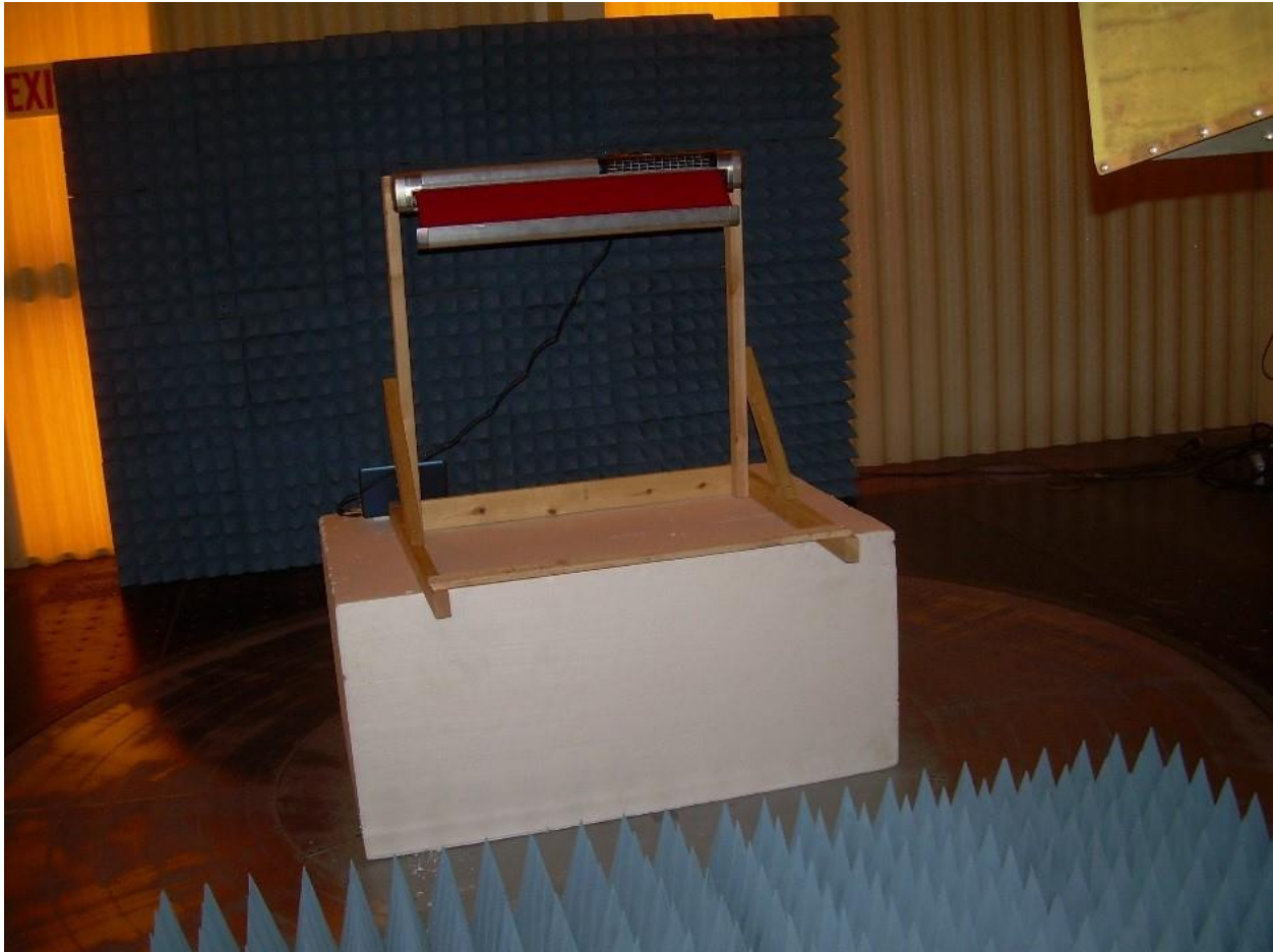
Photograph 3. Front View Radiated Emissions 1000 - 12400 MHz Range – Awning Extending
