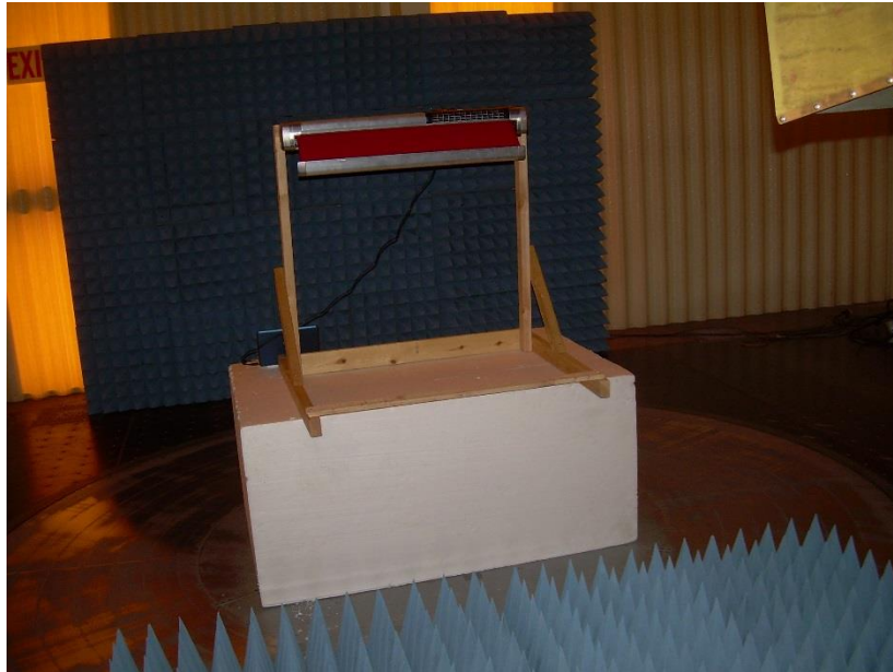
Photograph 3 - Front View Radiated Emissions – 1000 – 25000 MHz
