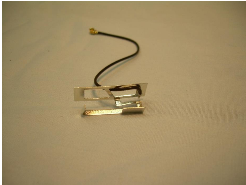
Photograph 10 – View of the Antenna
