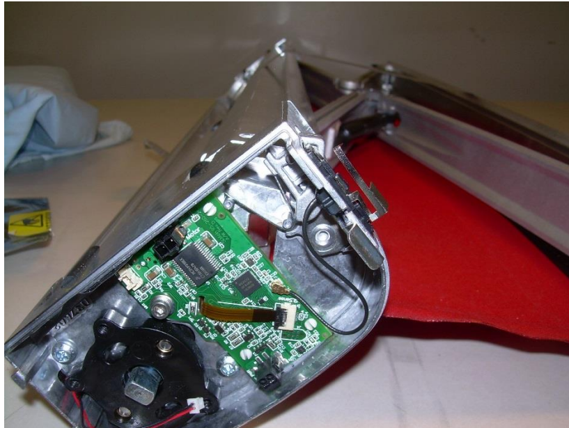
Photograph 9 – View with the End Cap and Motor Assembly Removed
