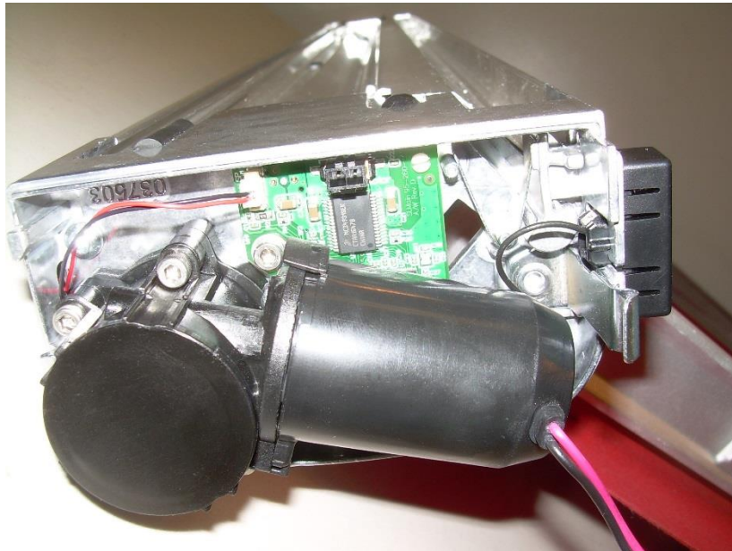
Photograph 8 – View with the End Cap Removed
