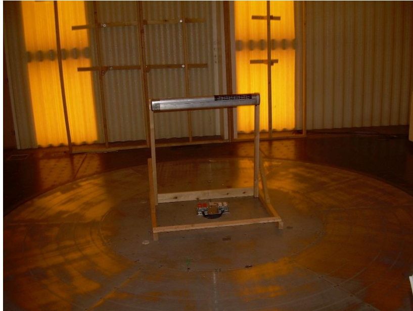
Photograph 1: Front View Radiated Emissions Below 30 MHz Shown with Awning Retracted
