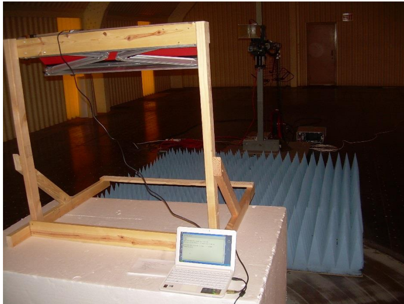
Photograph 4 - Back View Radiated Emissions – 1000 – 25000 MHz
