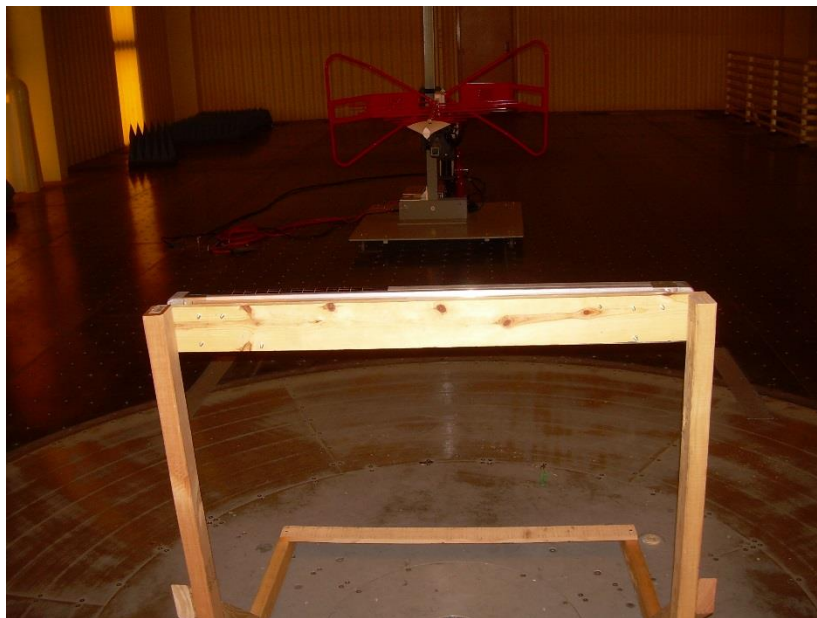
Photograph 2: Back View Radiated Emissions – 30 – 1000 MHz Shown with Awning Retracted
