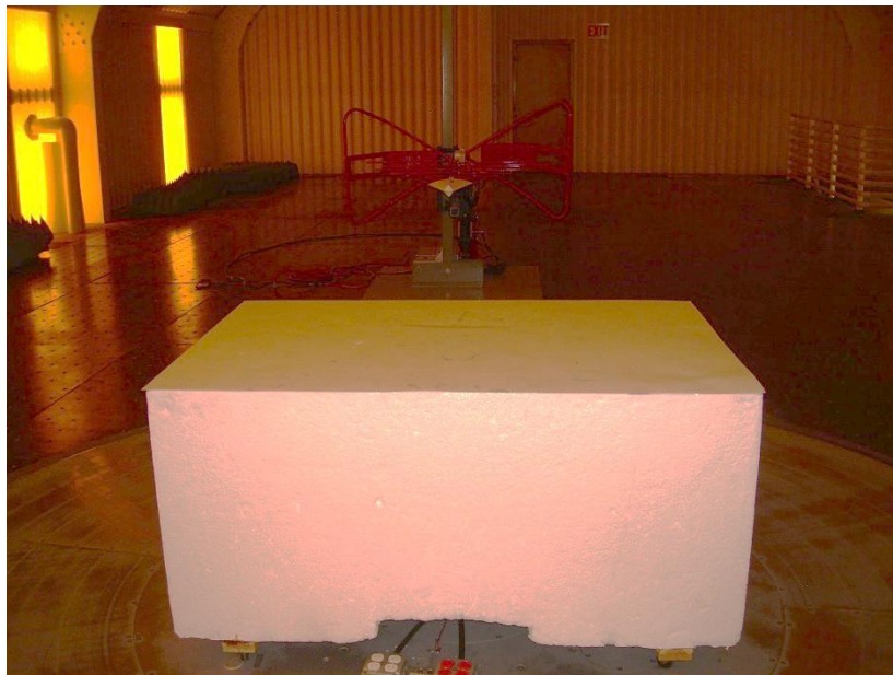
Photograph 18: Test Setup for Emissions from 30 MHz to 1000 MHz
