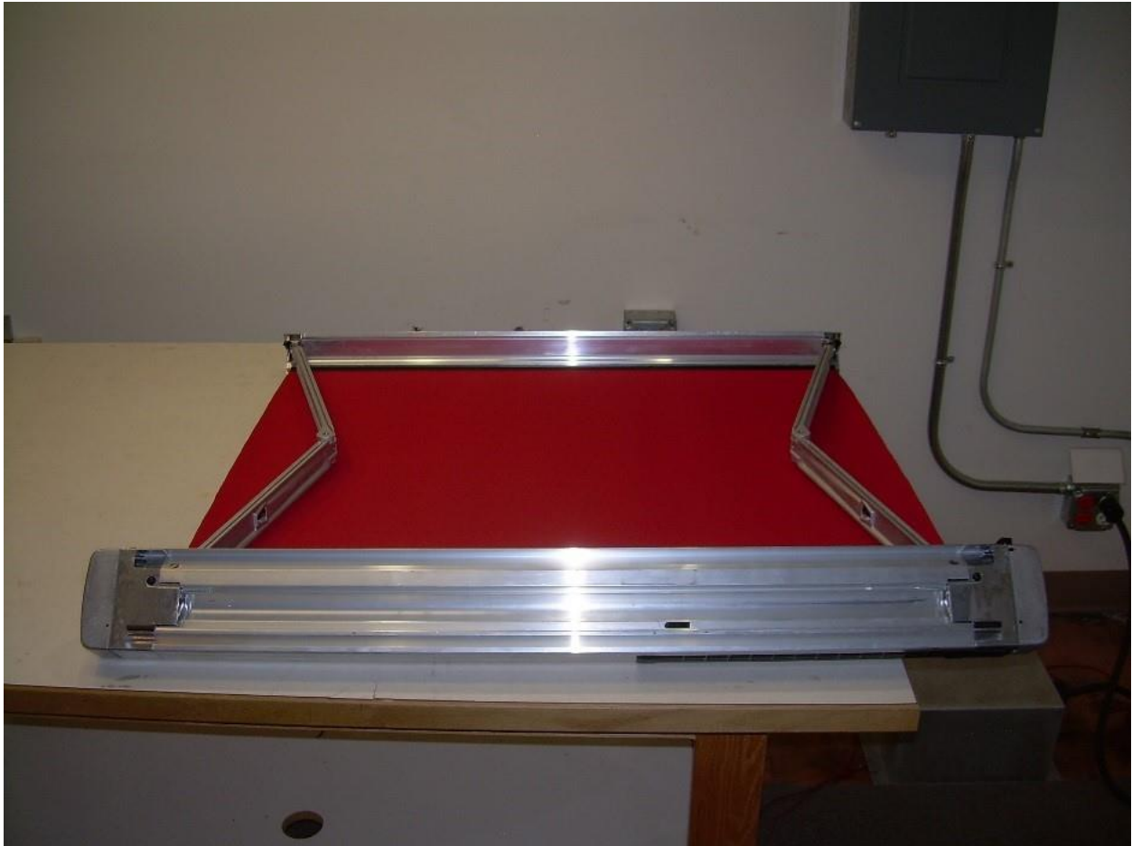
Photograph 5. Bottom Side of the EUT with Awning Extended
