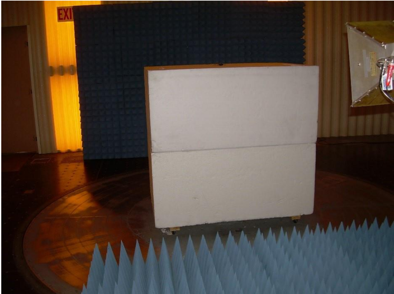
Photograph 3. Front View Radiated Emissions – Above 1000 MHz Configuration
