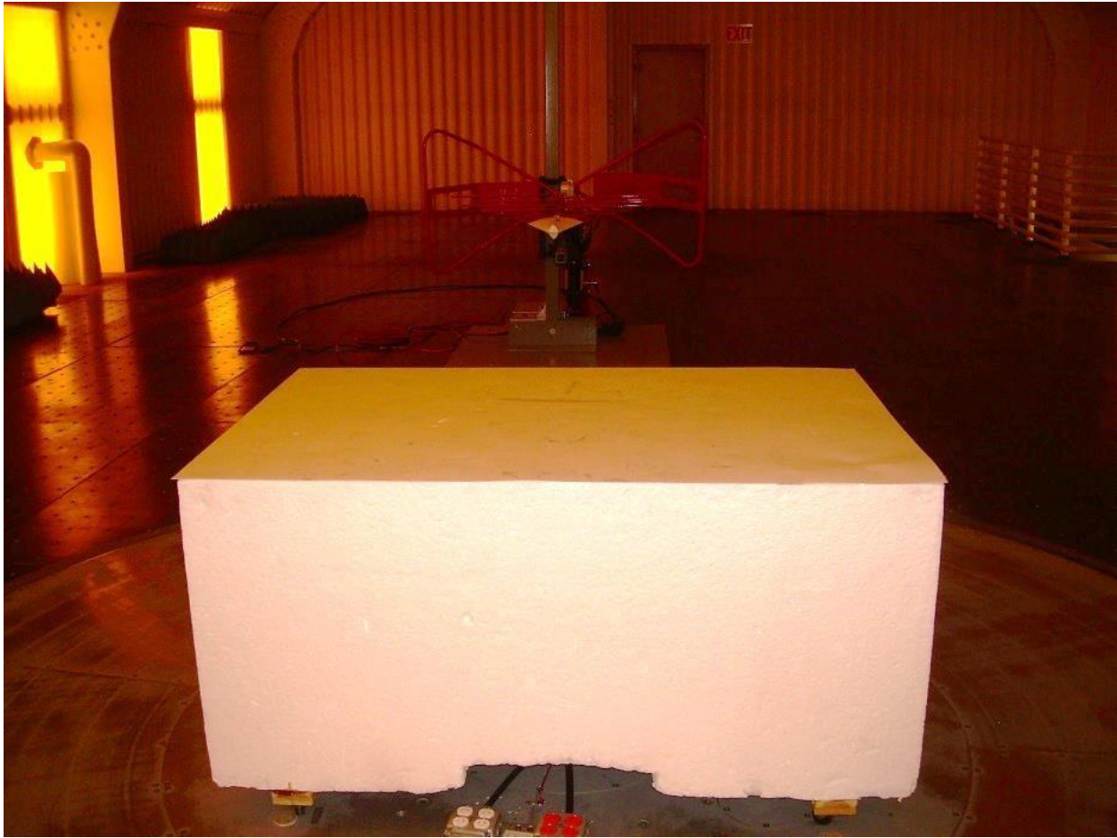
Photograph 9. Test Setup for Emissions From 30 MHz to 1000 MHz
