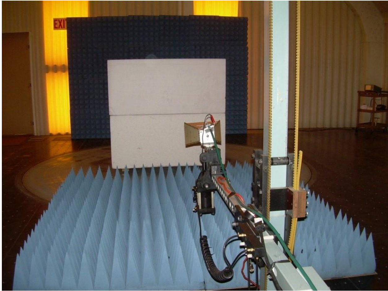
Photograph 10. Test Setup for Emissions Above 1000 MHz
