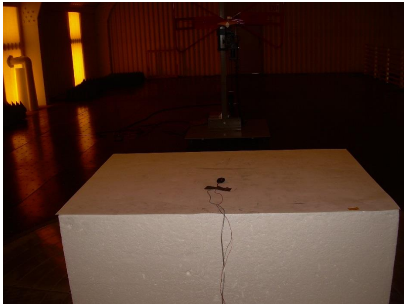
Photograph 2: Back View Radiated Emissions – Below 1000 MHz Configuration
