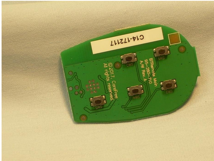
Photograph 12 – View of the Front Side of the PCB
