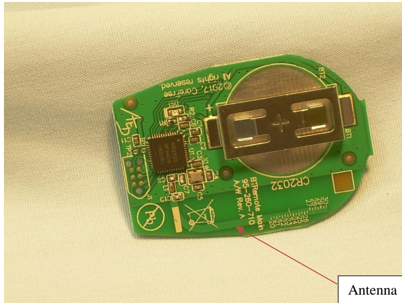
Photograph 13 – View of the Back Side of the PCB
