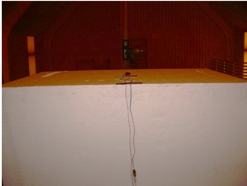
Photograph 4 – Back View Conducted Emissions – Above 1000 MHz Configuration
