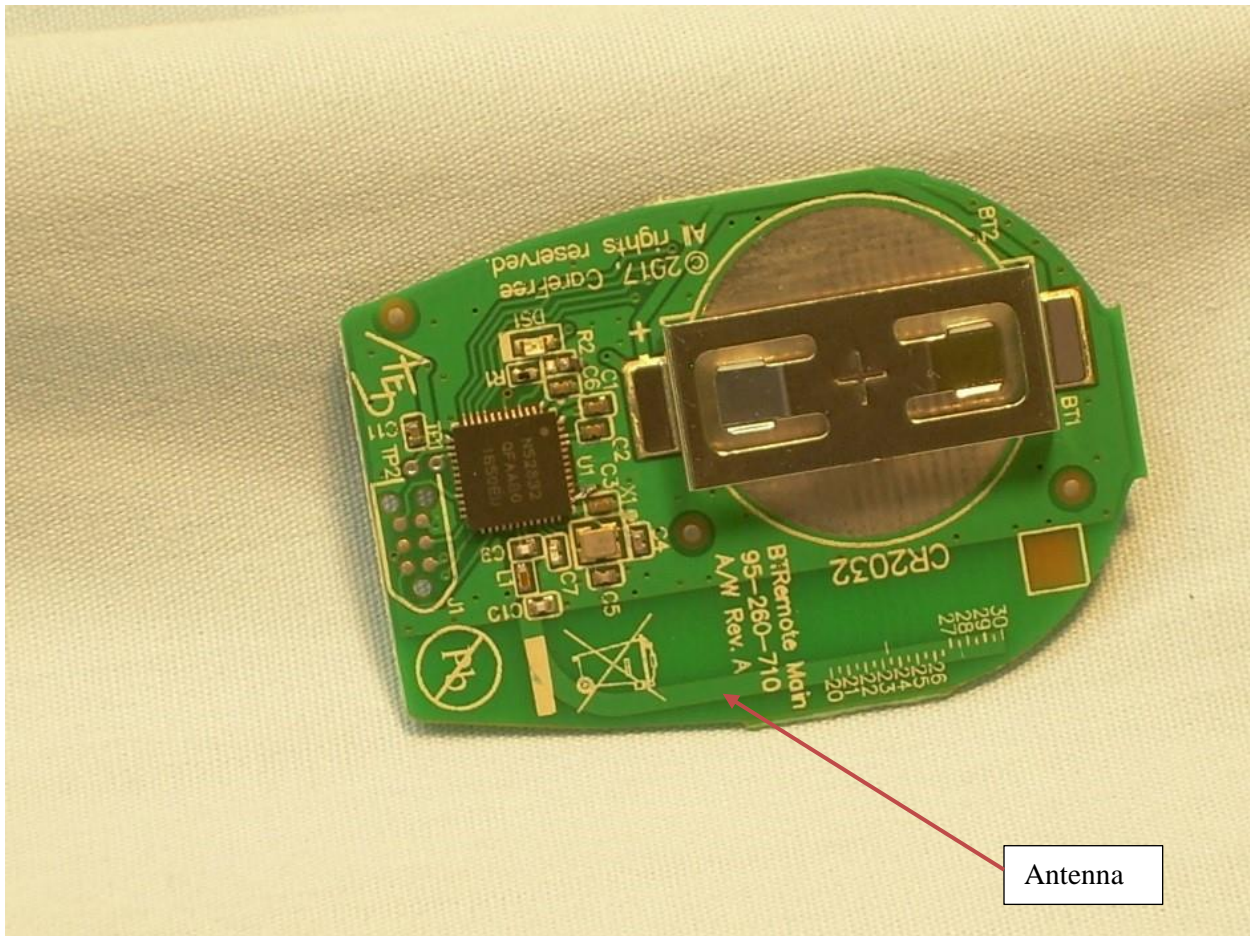
Photograph 4 – View of the Back Side of the PCB
