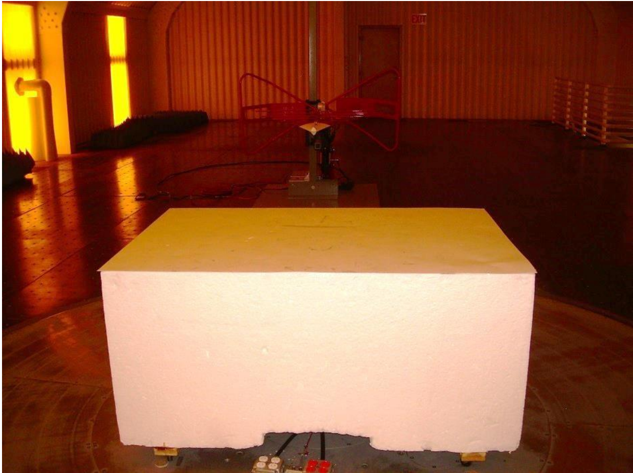
Photograph 11. Test Setup for Emissions From 30 MHz to 1000 MHz
