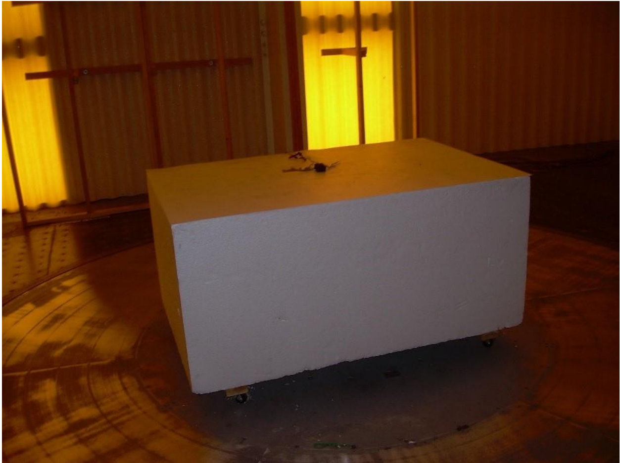
Photograph 3. Front View Radiated Emissions – Below 30 MHz
