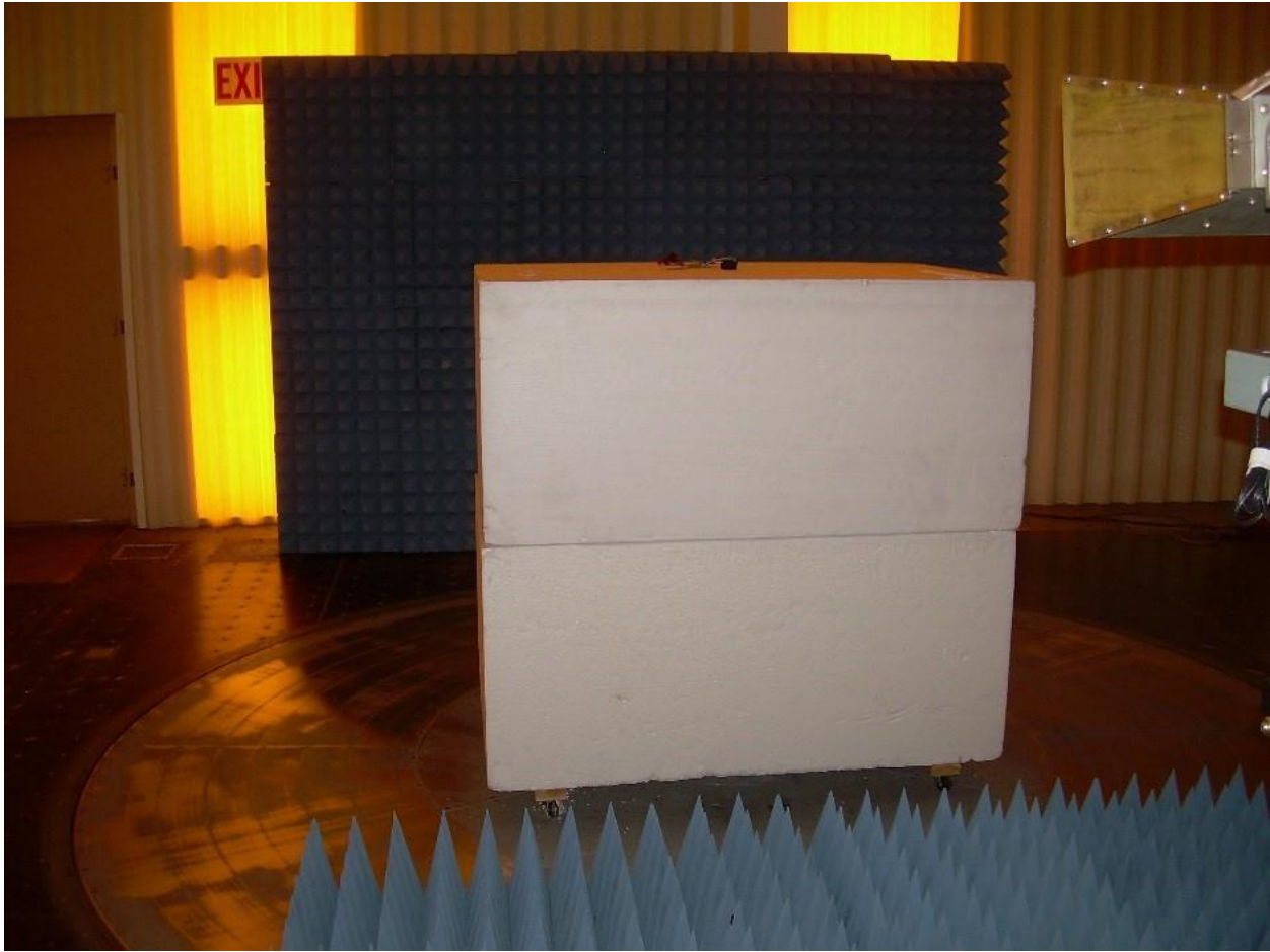
Photograph 5. Front View Radiated Emissions – Above 1000 MHz
