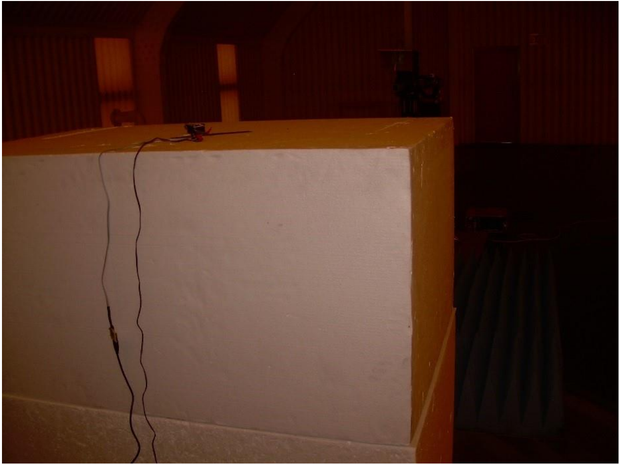
Photograph 6. Back View Radiated Emissions – 30 – 1000 MHz
