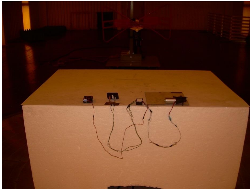
Photograph 4: Back View Radiated Emissions – 30 – 1000 MHz
