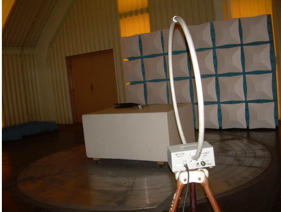
Photograph 1: Front View Radiated Emissions, Below 30 MHz Configuration
