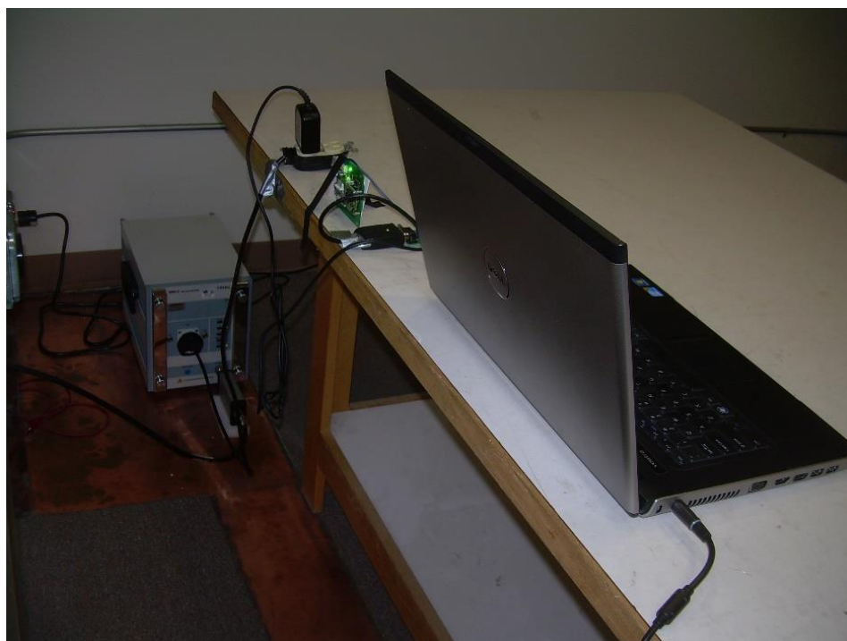
Photograph 8: Back View Conducted Emissions Configuration
