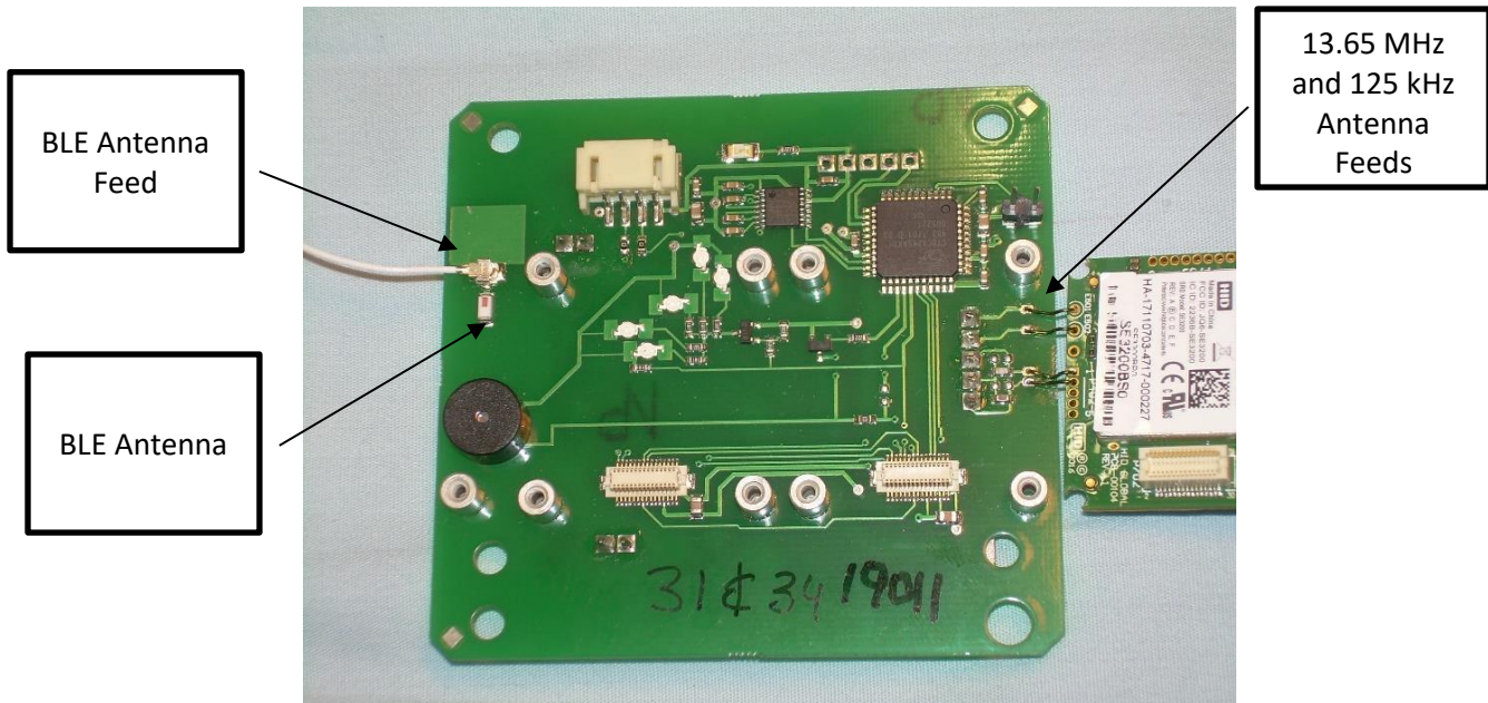
Photograph 3 – Front View with Modules Removed
