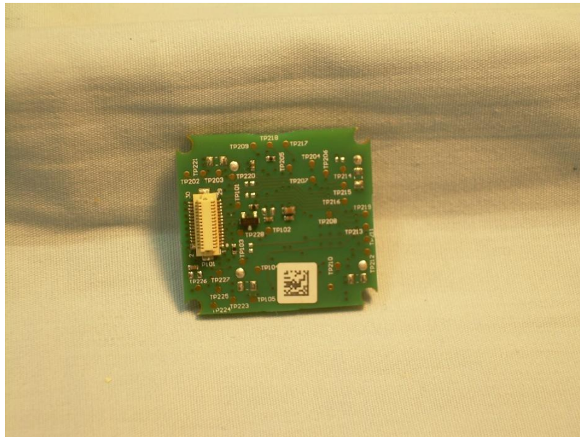
Photograph 7 – Back View RFID Module
