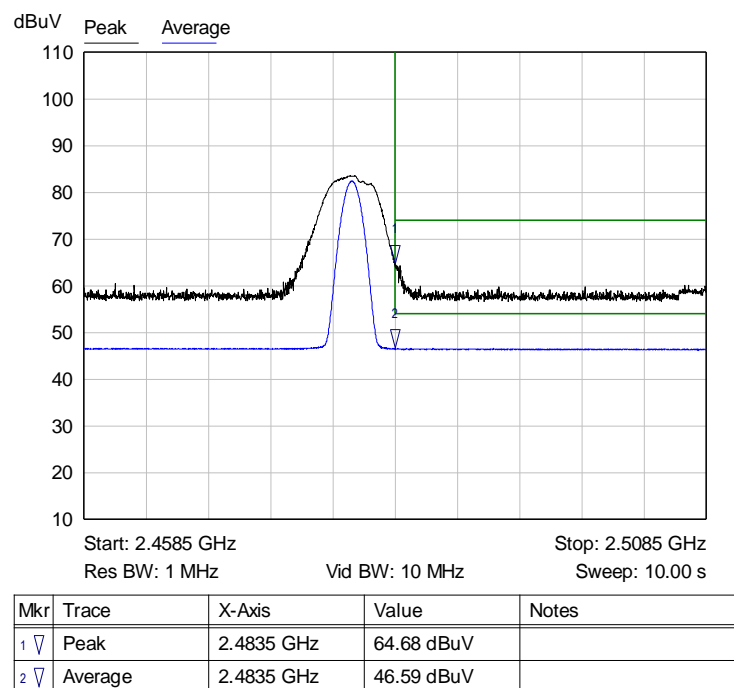
Graph 10: Radiated Upper Band Edge Plot
