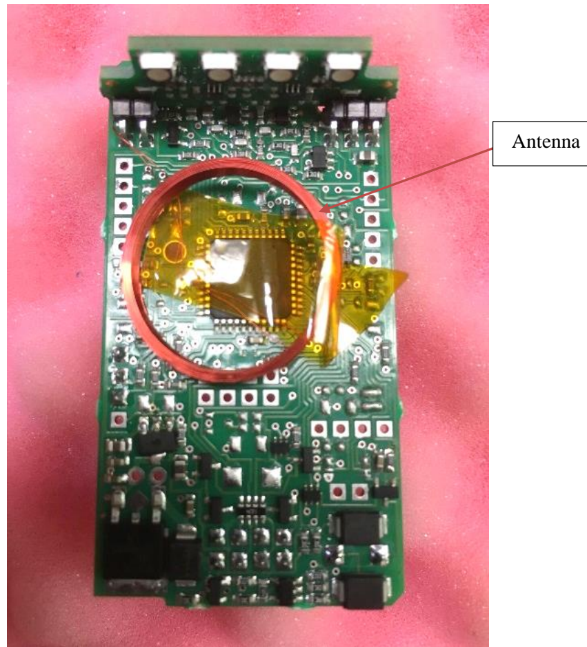
Photograph 1 – View of the Front Side of the EUT PCB
