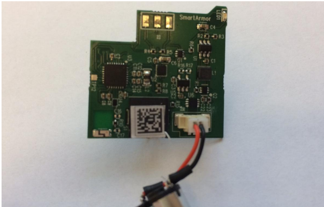
Figure 7: PCBA TOP
