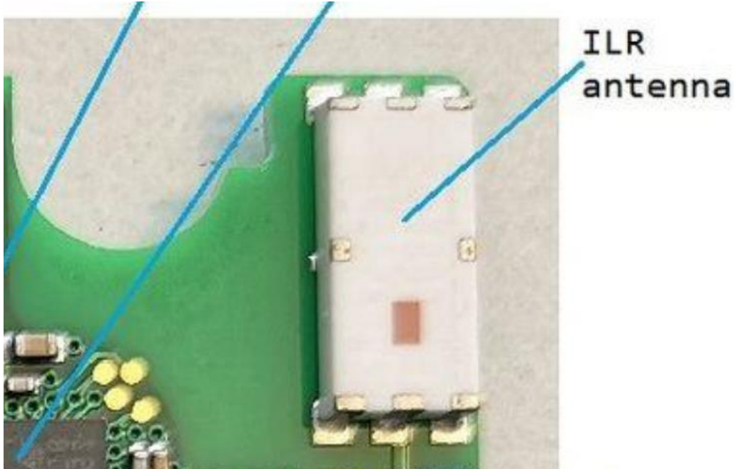
Photograph 3: EUT A, antenna view (provided by customer)
