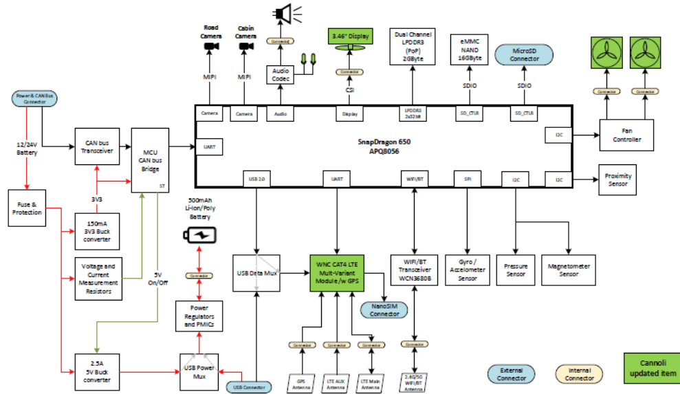
Figure 6: Block Diagram of Test Configuration
