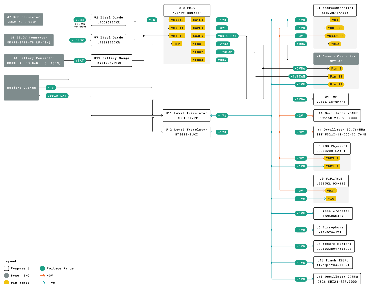
Nicla Vision Power Tree
