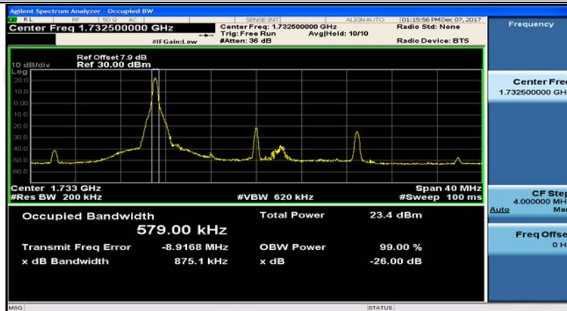
(Channel Bandwidth:20 MHz)_MCH_16QAM_1RB#50
