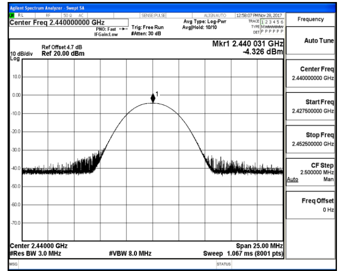
Channel 19 / 2440 MHz
