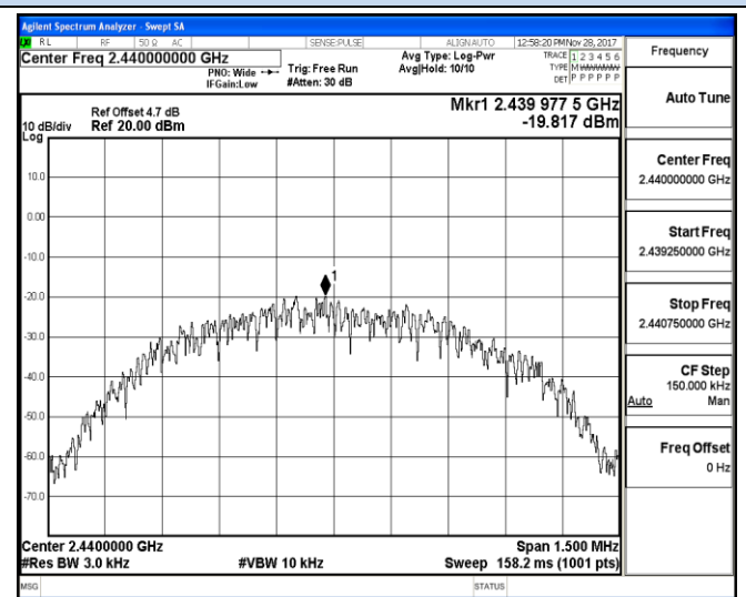
Channel 19 / 2440 MHz
