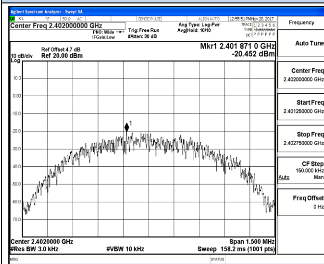
Channel 0 / 2402 MHz
