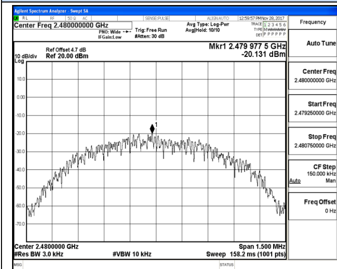
Channel 39 / 2480 MHz
