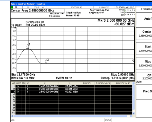
Channel 18 / 2480 MHz – Average
