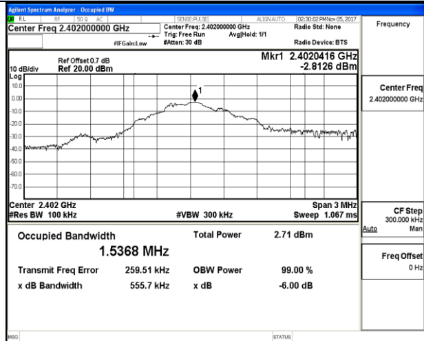
Channel 0 / 2402 MHz
