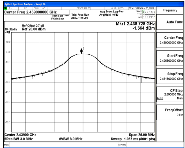
Channel 09 / 2439 MHz
