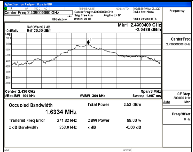
Channel 09 / 2439 MHz
