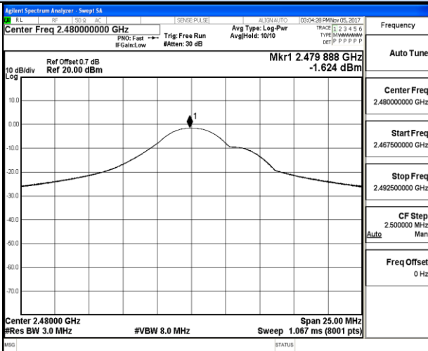
Channel 18 / 2480 MHz
