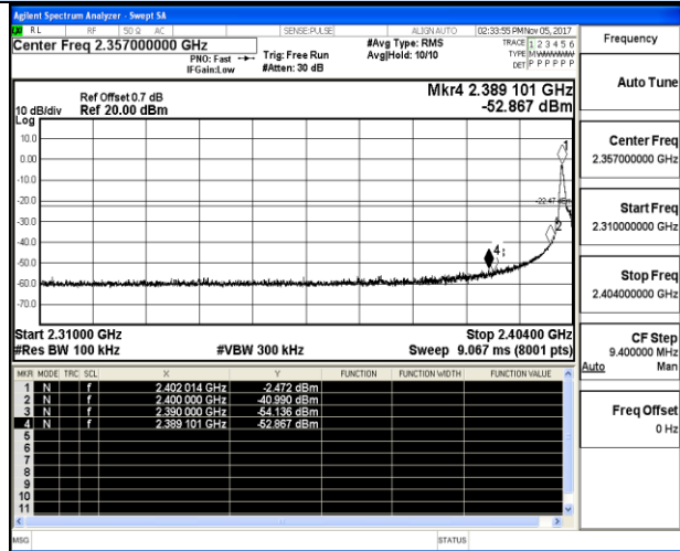
Channel 0 / 2402 MHz
