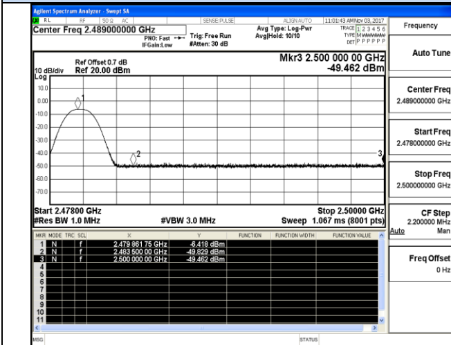
Channel 18 / 2480 MHz – Peak
