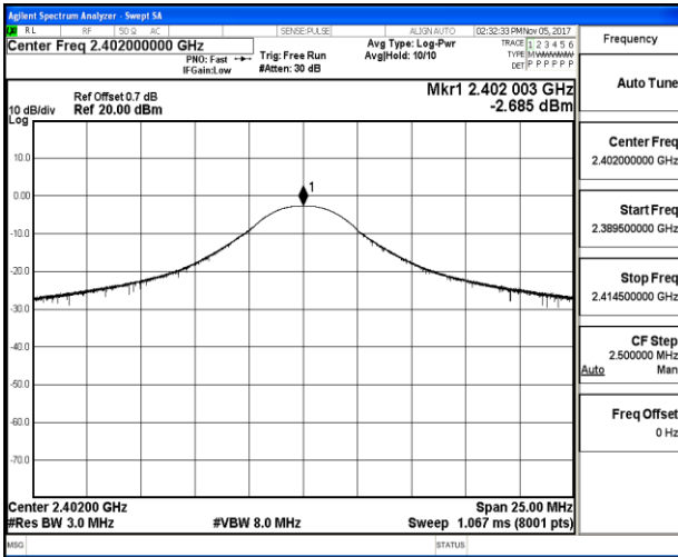
Channel 0 / 2402 MHz
