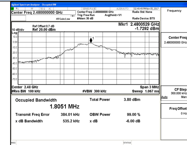
Channel 18 / 2480 MHz
