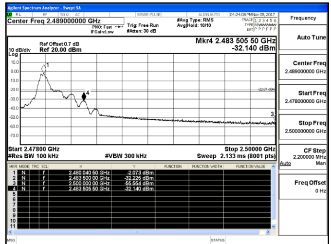
Channel 18 / 2480 MHz
