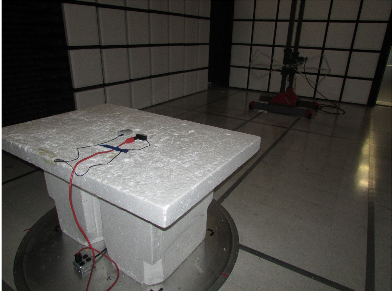
Figure 2: Radiated emissions <1GHz – Back view
