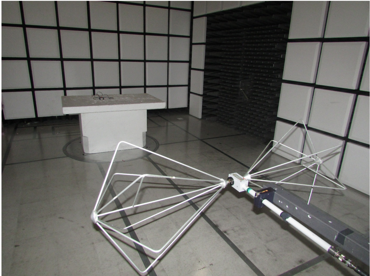
Figure 1: Radiated emissions <1GHz – Front view
