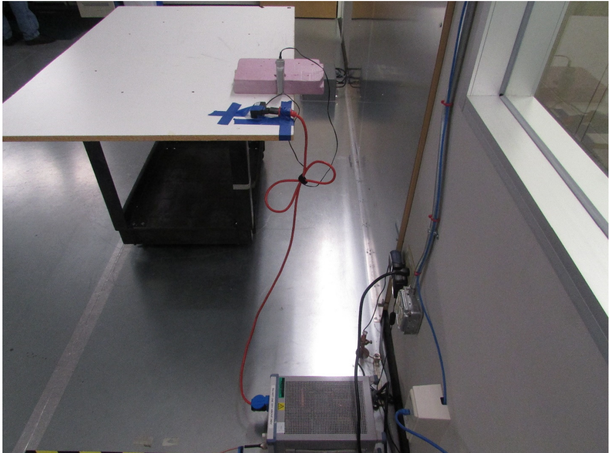
Figure 8: AC Conducted Emissions – Side view
