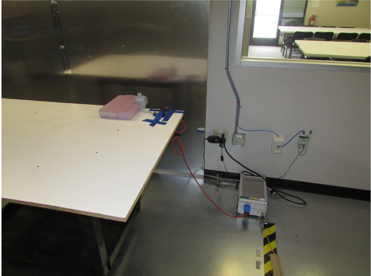
Figure 7: AC Conducted Emissions – Front view
