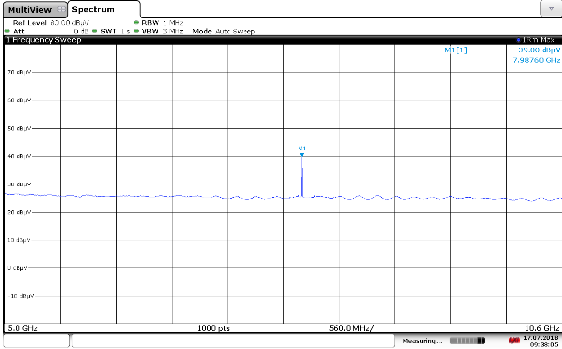
Figure 7.6.1.3-5: 5 GHz – 10.6 GHz
