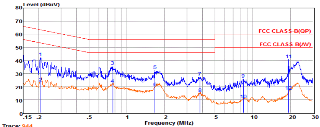
Trace: 944 Pol:
