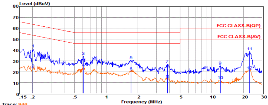
Trace: 946 Pol:
