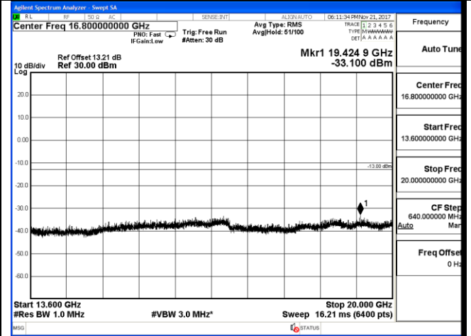
13.6 GHz – 20 GHz
