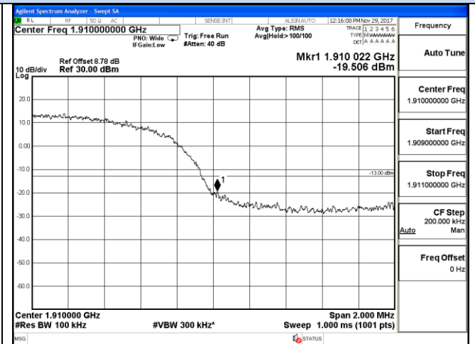
Channel 9538 / 1907.6 MHz
