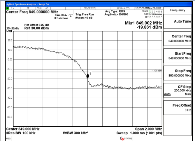
Channel 4233 / 846.6 MHz
