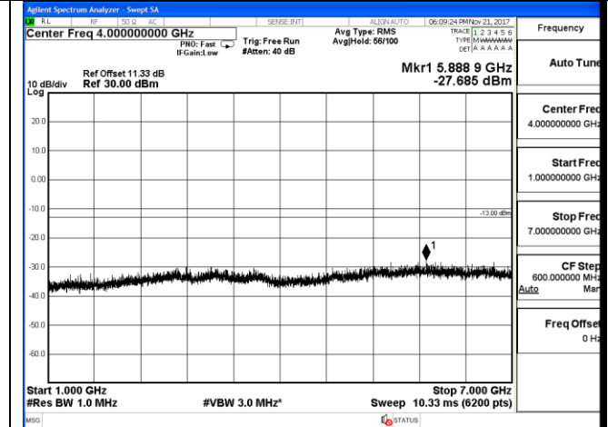
1000 MHz – 7000 MHz
