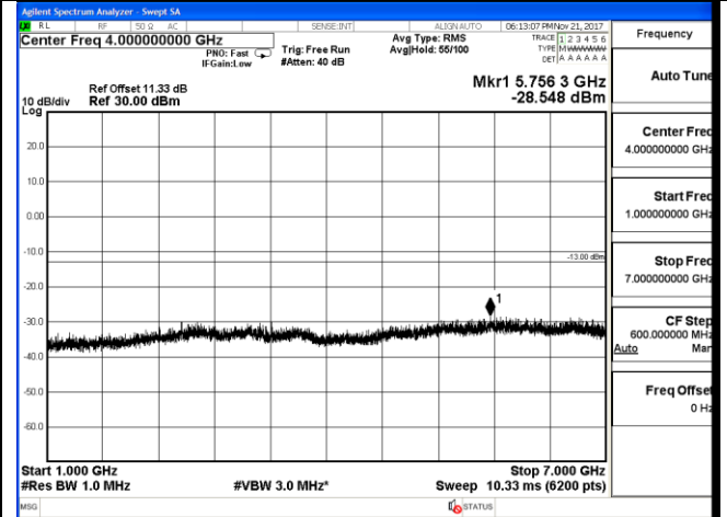
1000 MHz – 7000 MHz
