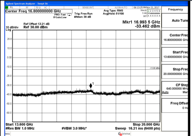
13.6 GHz – 20 GHz
