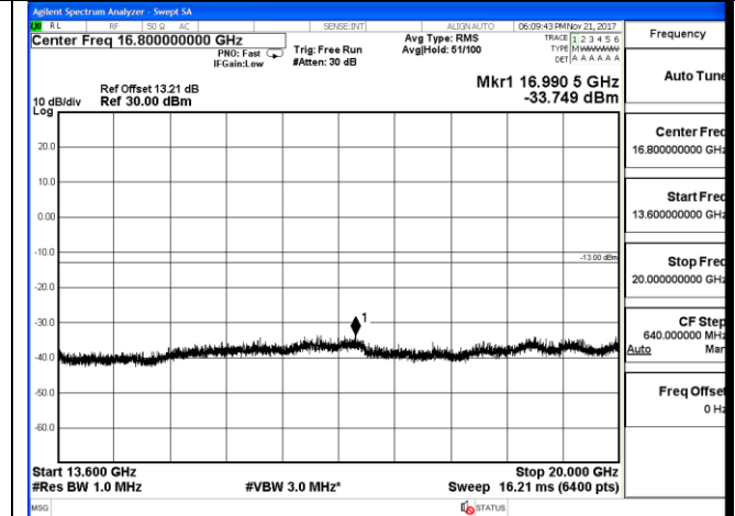
13.6 GHz – 20 GHz
