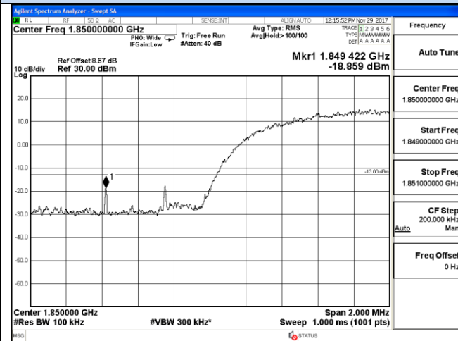
Channel 9262 / 1852.4 MHz
