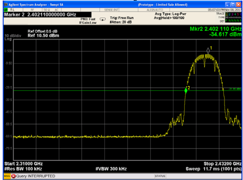
TX 11b: Band edge-left side
