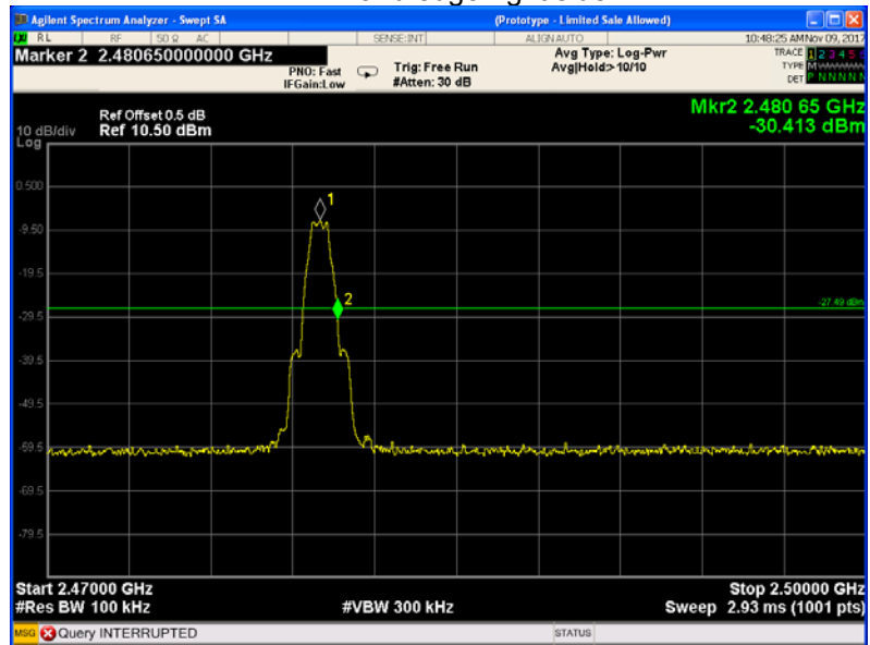
BLE: Band edge-right side
