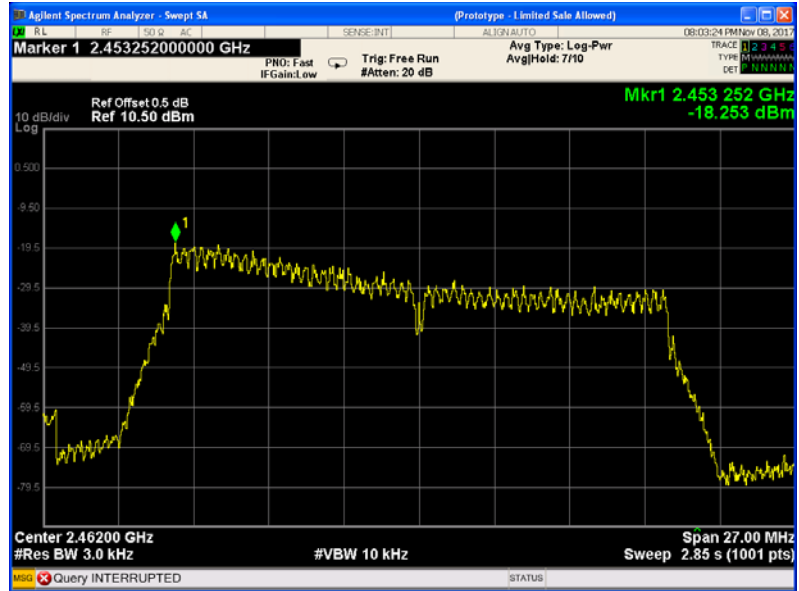
Mode: TX 11n HT20 channel 11
