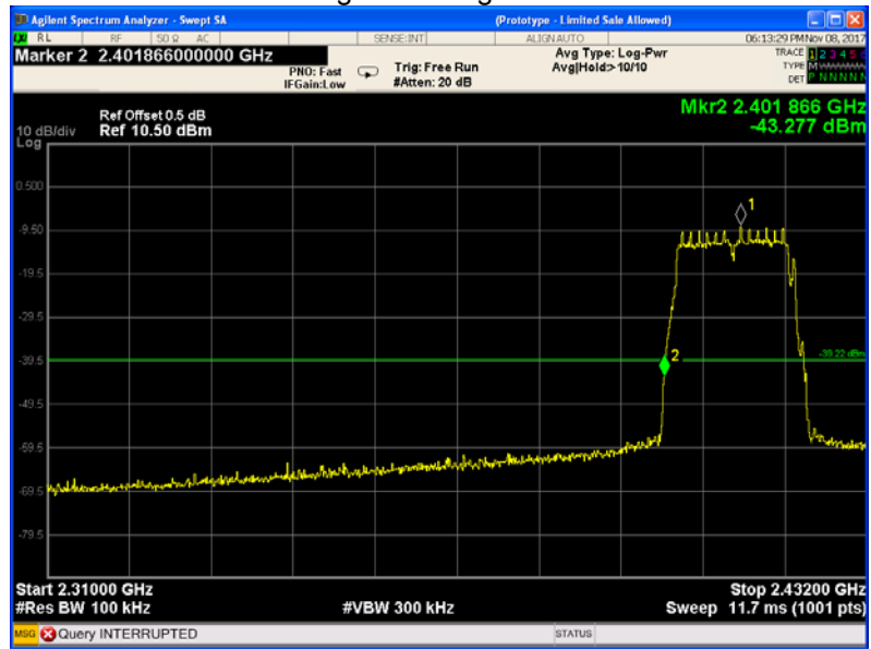
TX 11g: Band edge-left side
