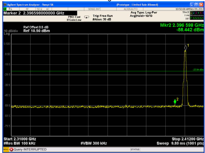
BLE: Band edge-left side
