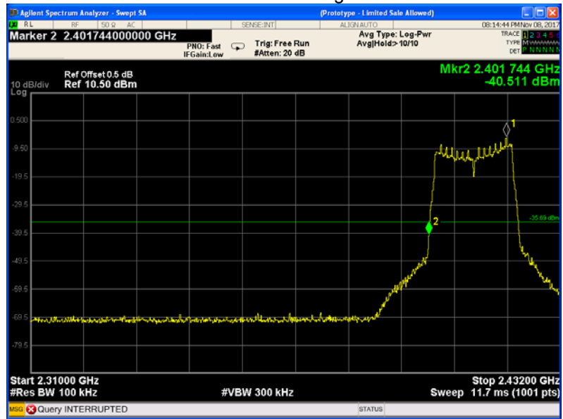
TX 11n HT20: Band edge-left side
