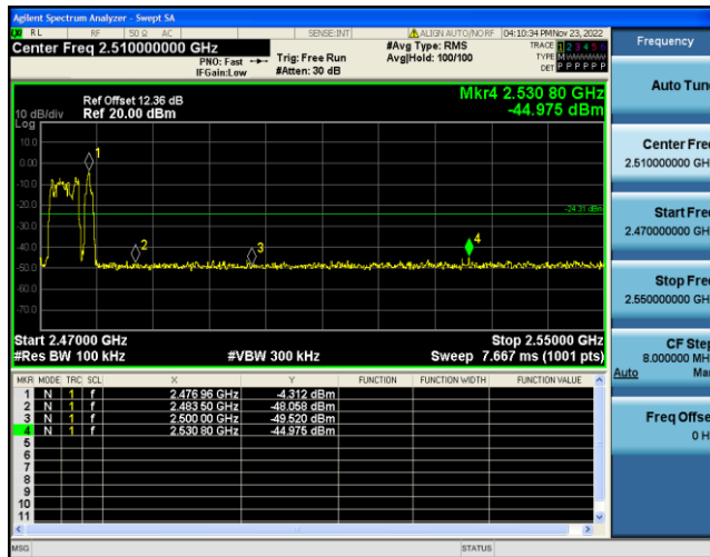
3DH5-Ant1-High-Hop_2480--4.31
