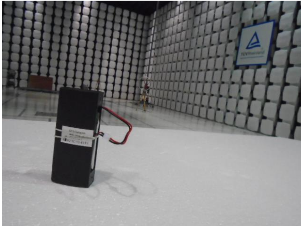
Figure 7: Test Setup for 9 kHz to 30 MHz (Front View)
