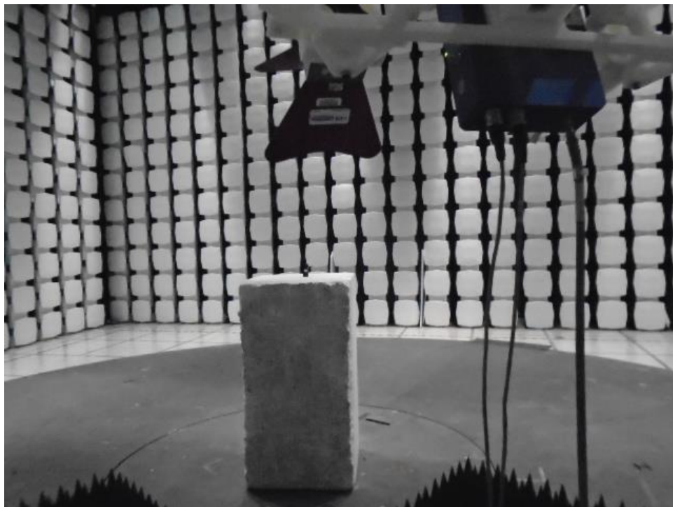
Figure 12: Test Setup for 1GHz to 26.5GHz (Rear View)
