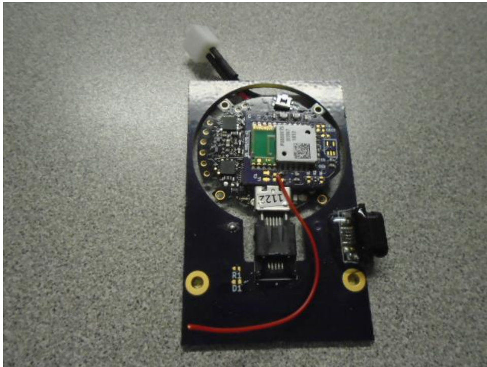
Figure 1: Internal (Front View)
