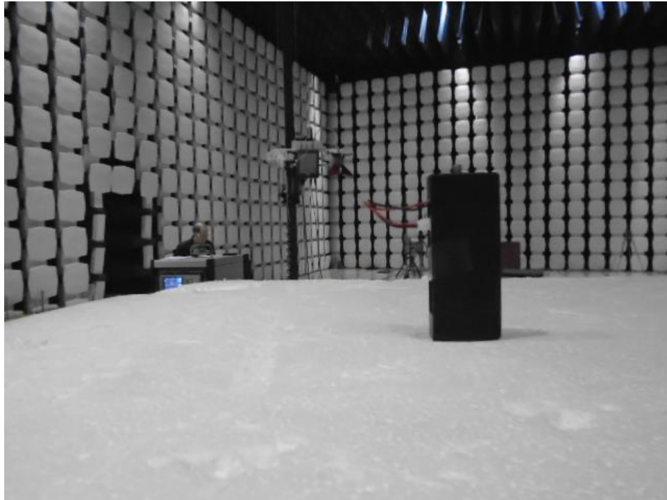
Figure 11: Test Setup for 1GHz to 26.5GHz (Front View)
