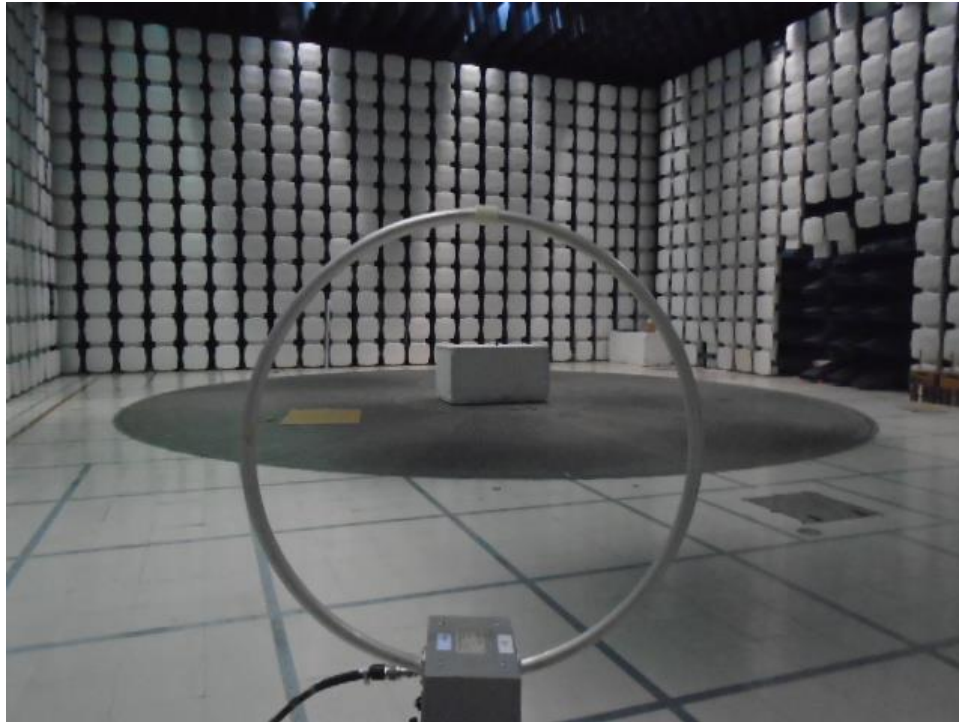
Figure 8: Test Setup for 9 kHz to 30 MHz (Back View)
