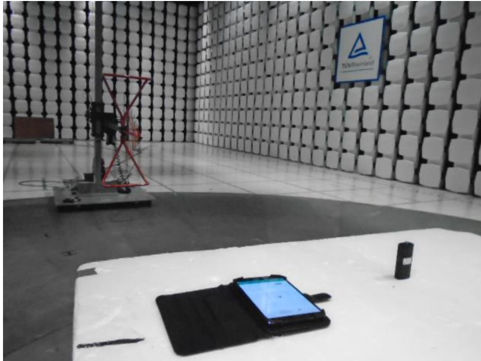
Figure 9: Test Setup for 30 MHz to 1000MHz (Front View)
