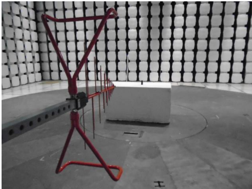
Figure 10: Test Setup for 30 MHz to 1000MHz (Rear View)
