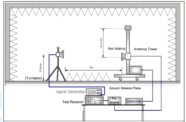
EIRP Test Setup
