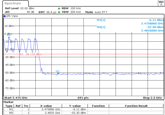
8-DPSK: Band Edge-High Channel (Hopping Mode)
