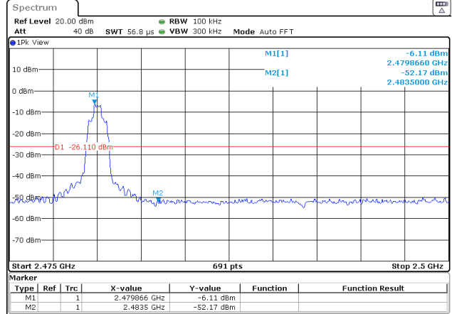
8-DPSK: Band Edge-High Channel
