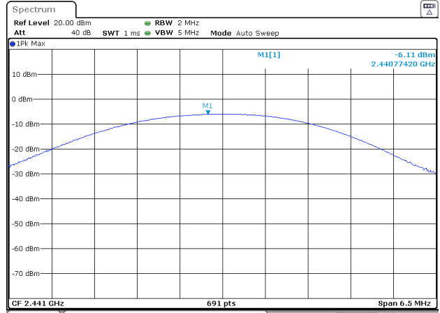
Peak output Power plot on channel 39 (2Mbps)
