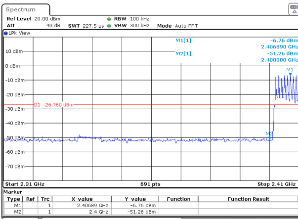
8-DPSK: Band Edge-Low Channel (Hopping Mode)
