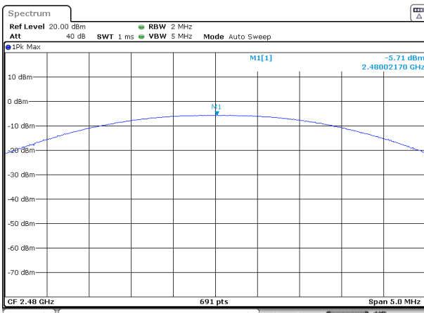
Peak output Power plot on channel 78 (1Mbps)
