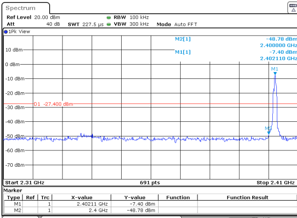
8-DPSK: Band Edge-Low Channel
