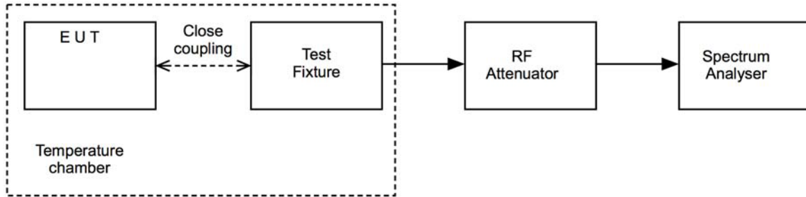
Figure iv Test Setup
