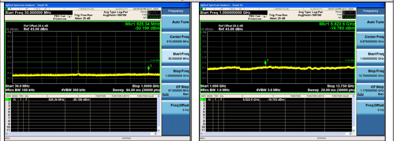
25kHz, FM modulation, Assigned Frequency:467.6500MHz, 4.5W
