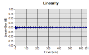
Linearity +/-1.87% (+/-0.08dB)
