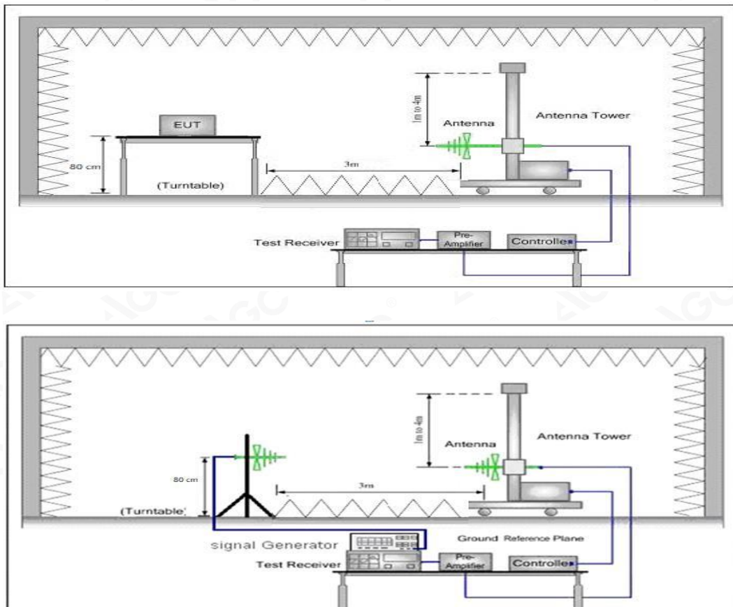
Radiated Below1GHz
