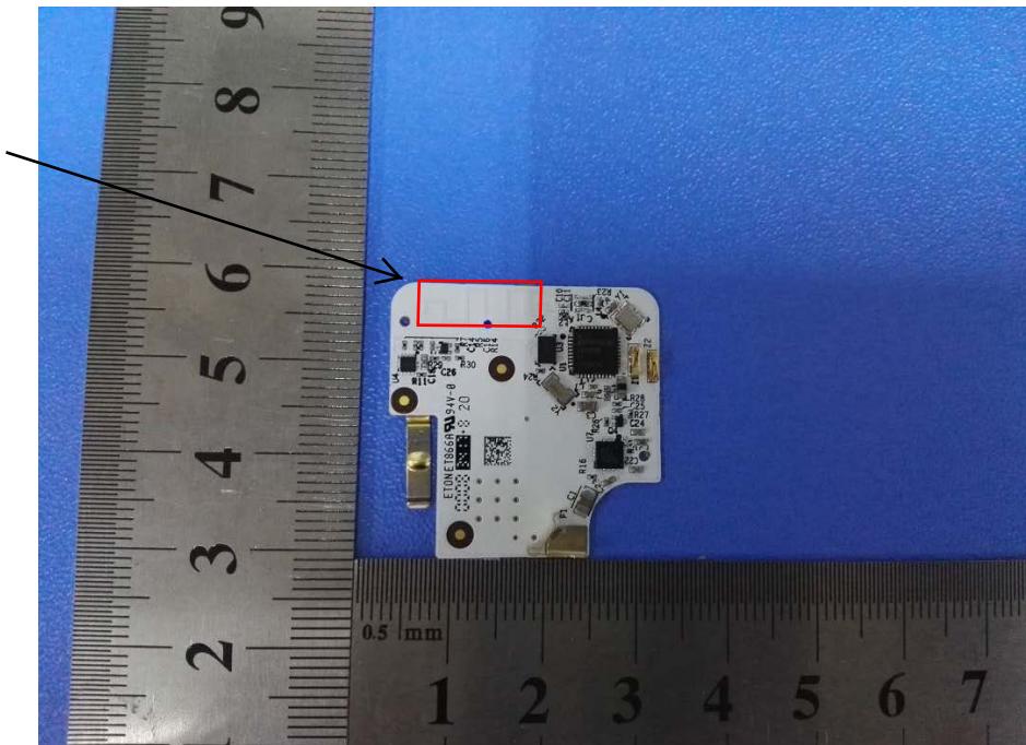
INTERNAL PHOTO OF SAMPLE – 4
